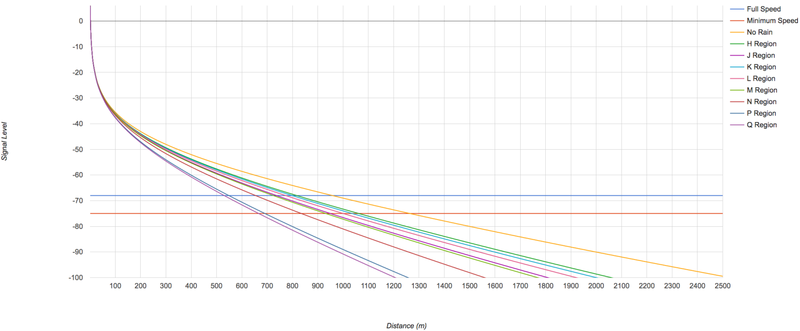
MetroLinq Availability vs. Distance (ML-60-S-30-18 to ML-60-35), H-Q, 99.9%
