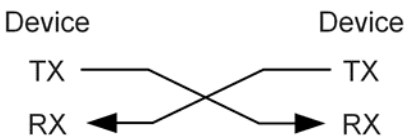
Figure 7-1 Optical Cable Connections
